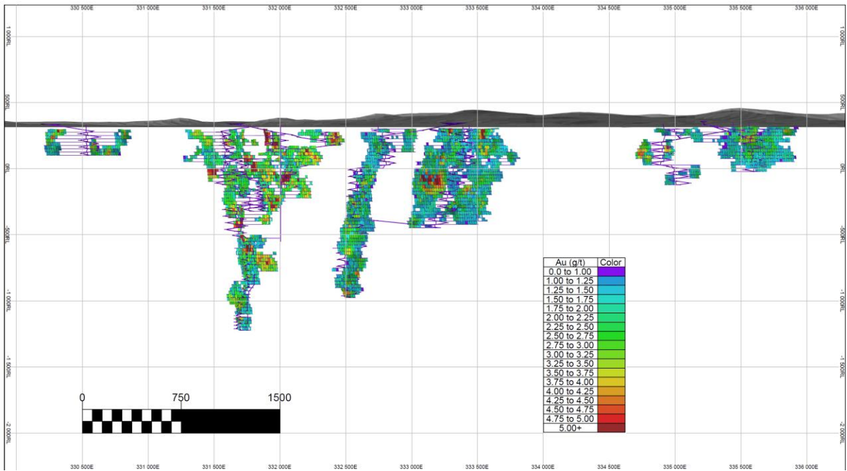
Figure 1: Conception minière
